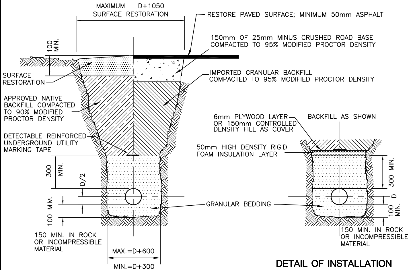
ORDINARY BEDDING DETAIL
