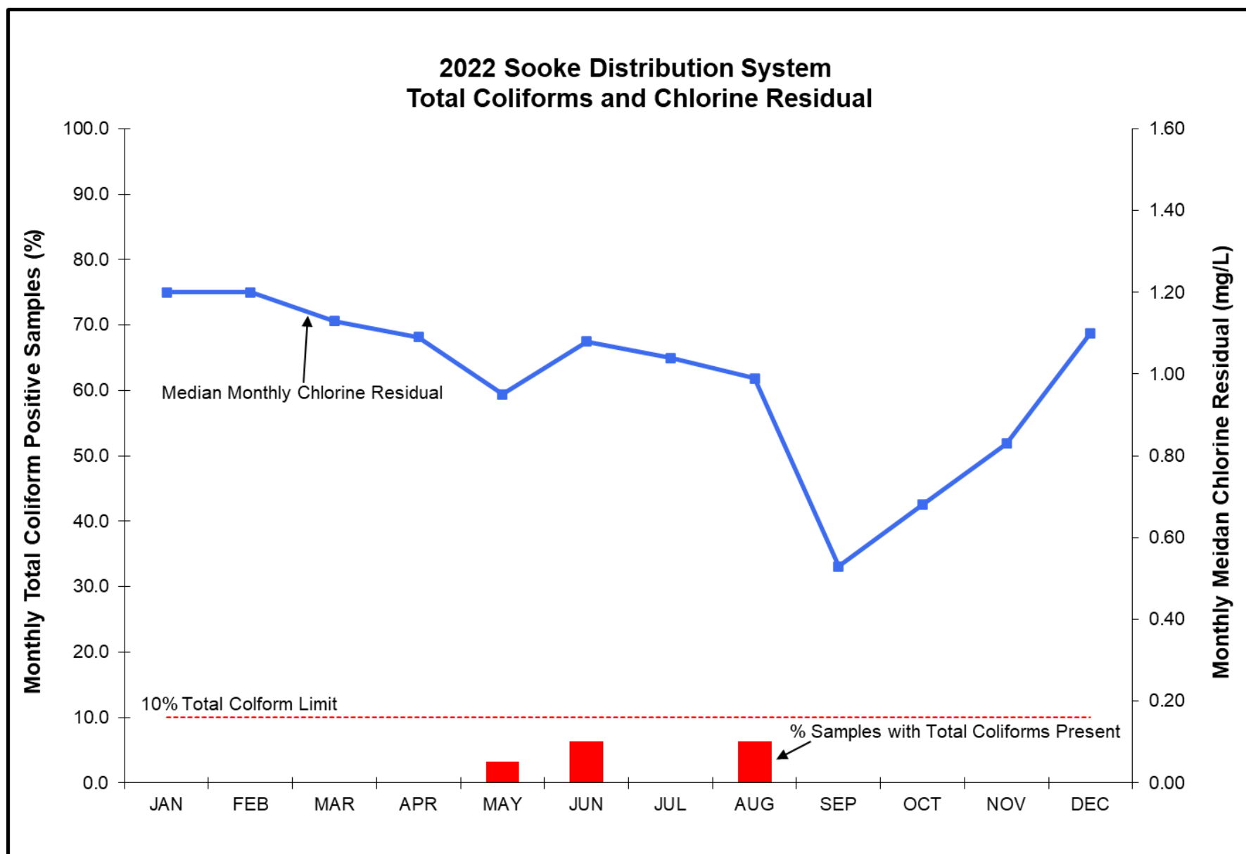
Figure 31 Sooke/East Sooke Distribution System Total Coliforms and Chlorine Residual in 2022
