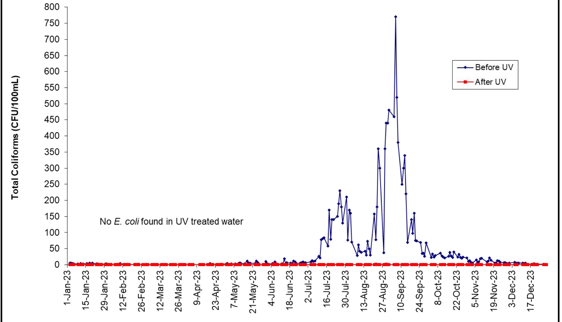
Figure 26 2023 UV Treated Water at Goldstream Water Treatment Plant Total Coliforms Before and After UV Treatment
