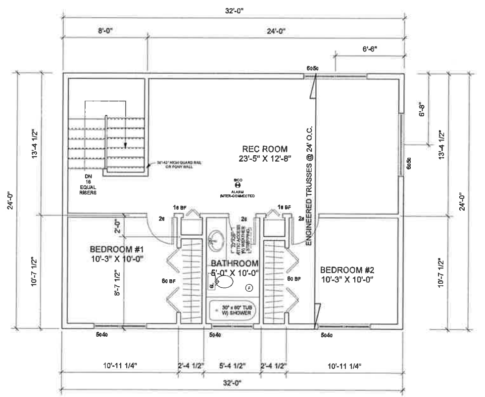
UPPER FLOOR PLAN SCALE: 1/4" = 1'0" AREA 705 SQ. FT.
