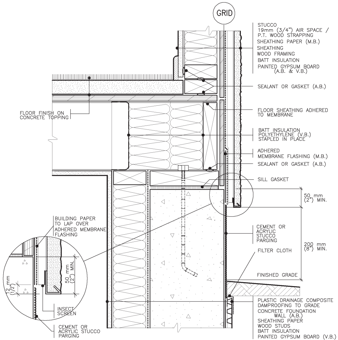
BASE OF WALL / FOUNDATION AIRTIGHT DRYWALL APPROACH
