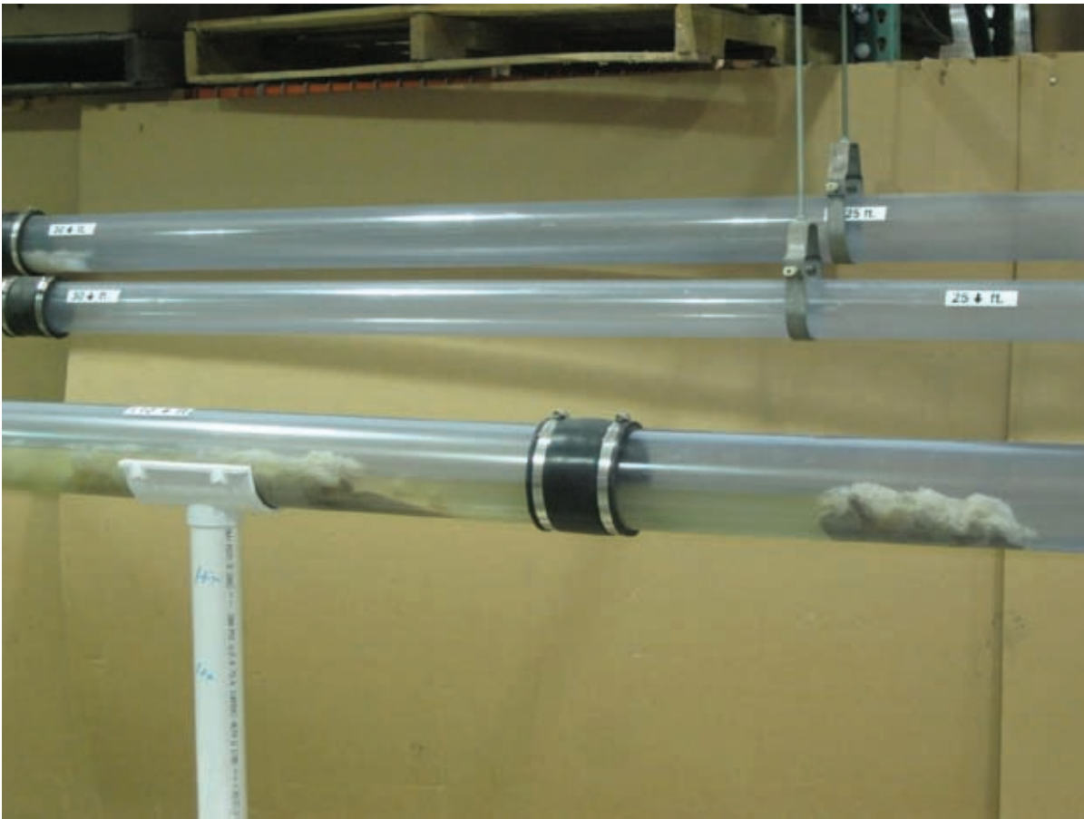
PHOTO 7-E ORDERLY FLOW OF SOLIDS IN TEST RUN #3 @ 1.28 GALLON (4.8 L) VOLUME, 1% SLOPE
