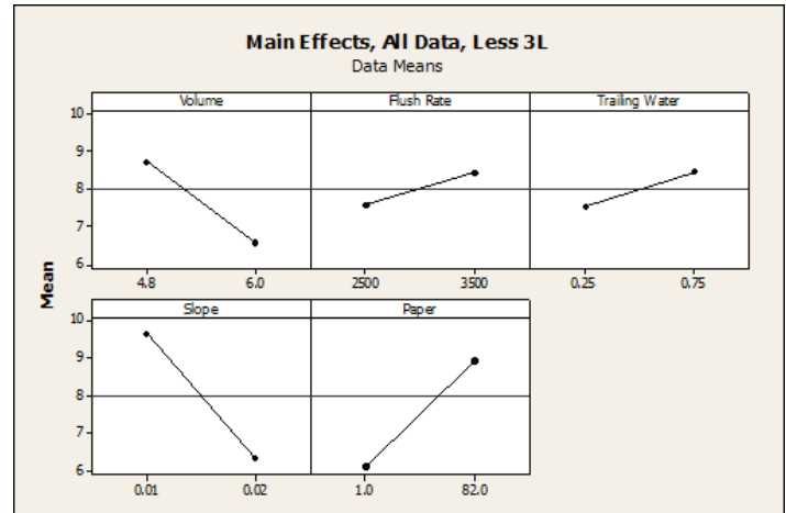
FIGURE 1. PRIMARY MAIN EFFECTS PLOT ALL DATA AND RESPONSE TABLE FOR MEANS
