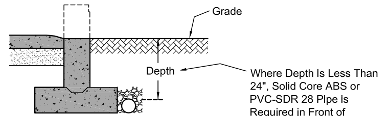
Detail @ Garage Door
