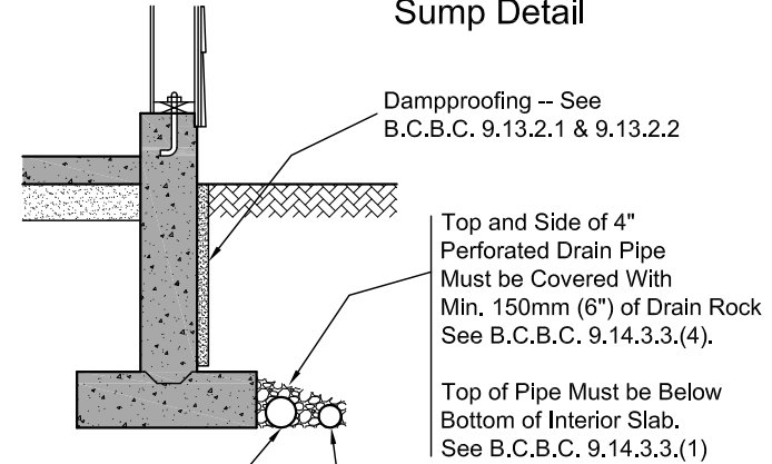
Footing Detail
