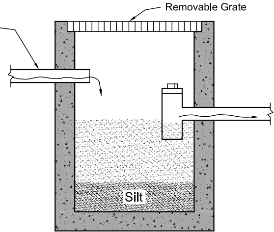
Sump Detail
