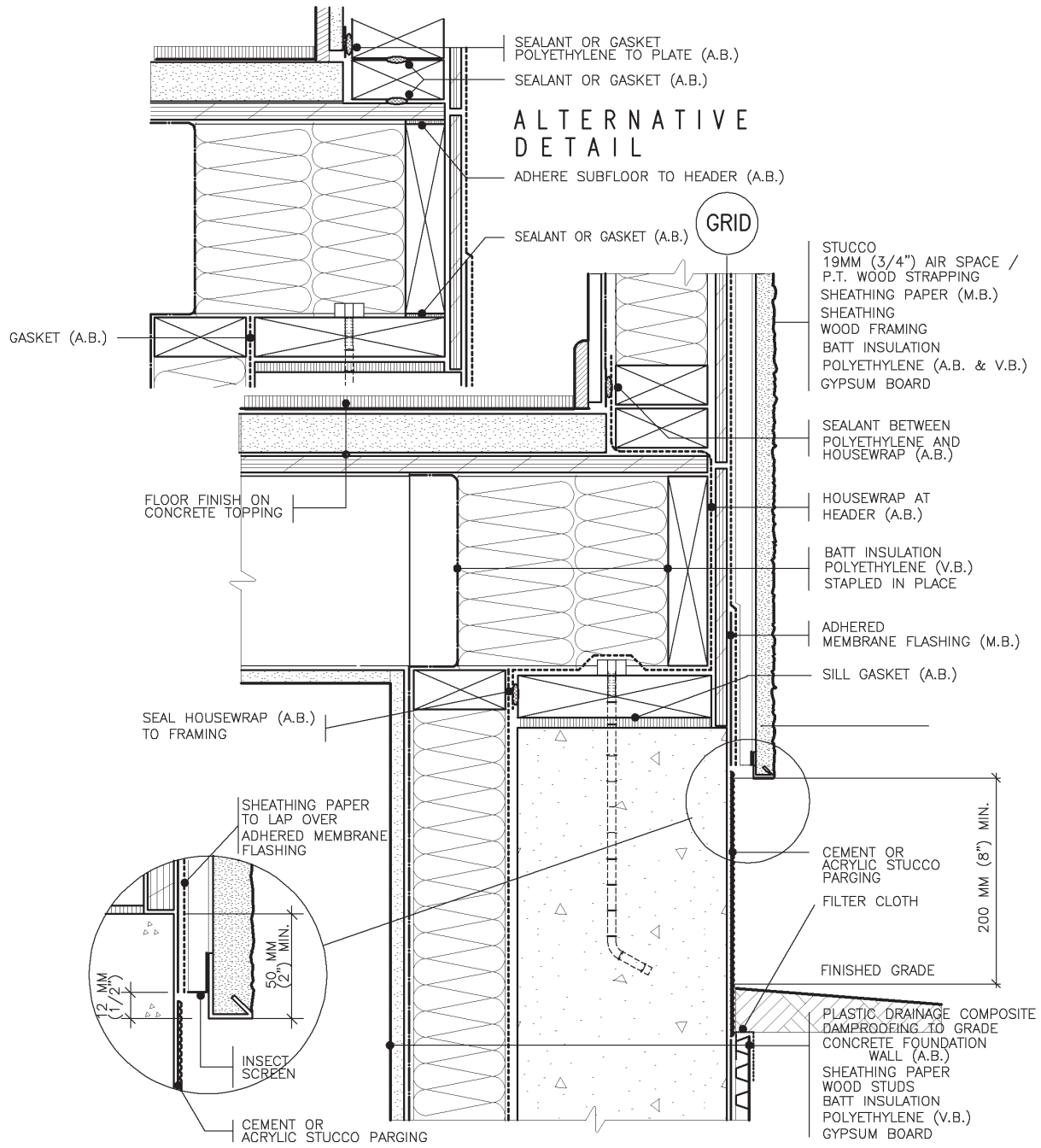
BASE OF WALL / FOUNDATION 2SPA SEALED POLYETHYLENE APPROACH 1" 0 4" 8" 50MM 0 100 200MM
