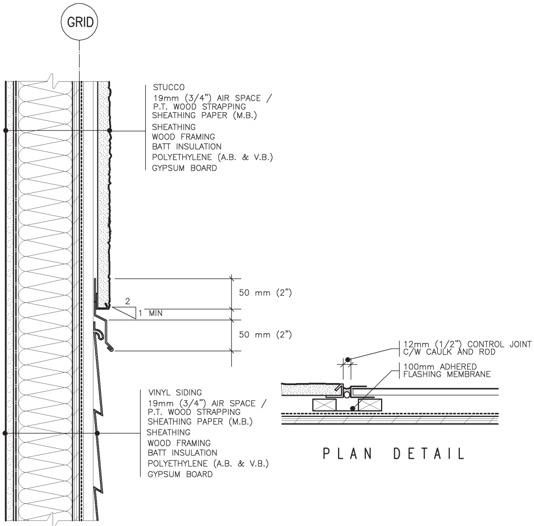
SECTION DETAIL
