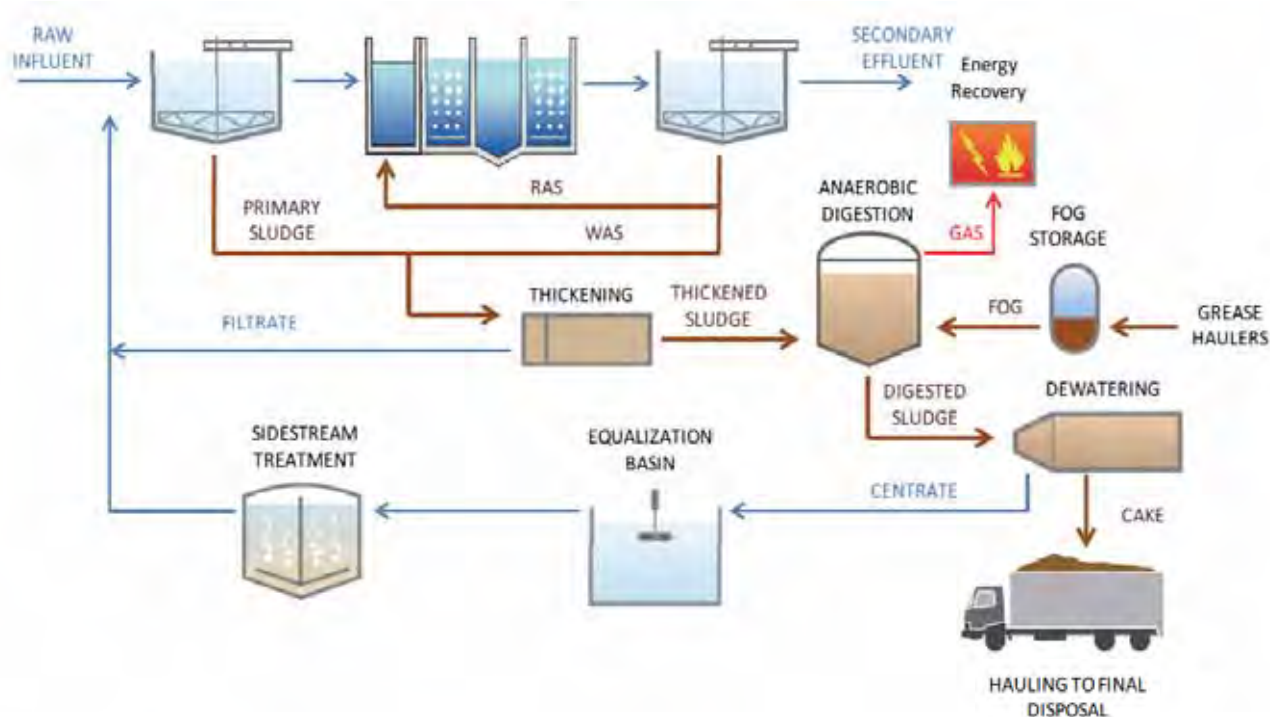
Figure 2.7 – Anaerobic Digestion
