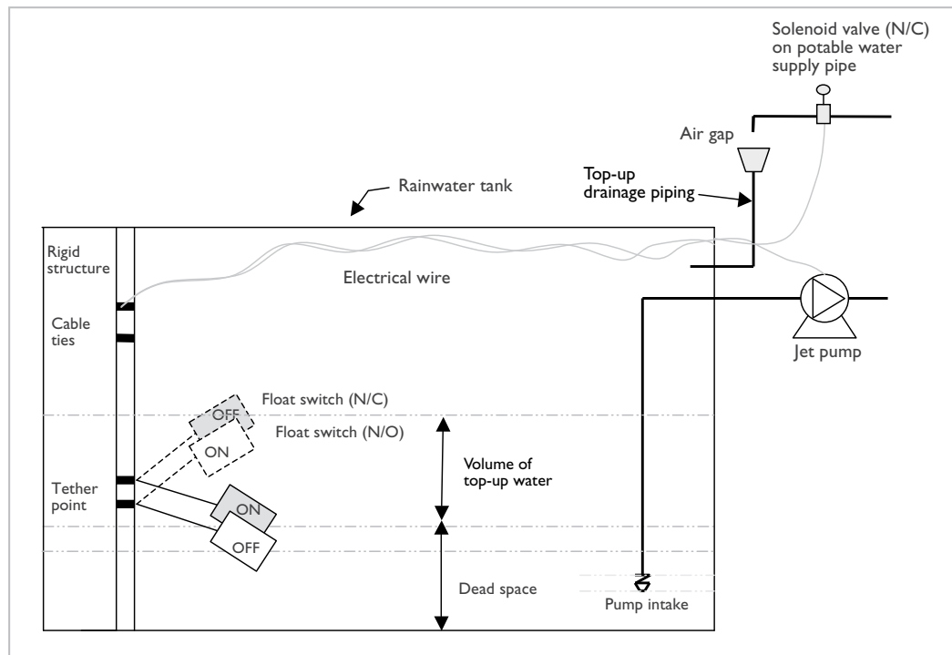
Figure 4-1 Components of an automatic top-up system
