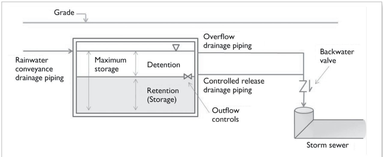
Figure D-1 RWH system with outflow controls and controlled release drainage piping for stormwater management. ('DETENTION' is the volume of runoff to be slowly released to storm sewer. The remaining volume 'RETENTION' is used to supply rainwater to permitted fixtures.)
