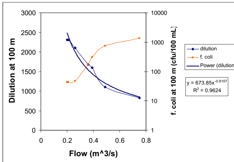
Figure 6.1 Diffuser dilution curve for 14 ports, and corresponding fecal coliform concentrations at the edge of the IDZ for minimum dilution conditions, for the Saanich East WWTP.
