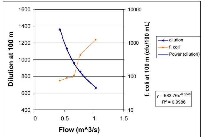
Figure 6.3 Diffuser dilution curve for 26 ports, and corresponding fecal coliform concentrations at the edge of the IDZ for minimum dilution conditions, for the West Shore WWTP.
