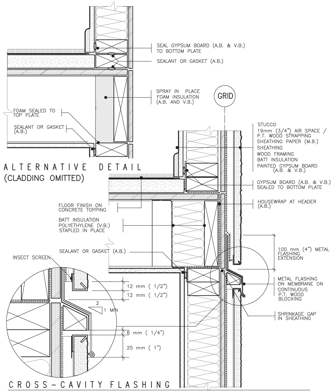
RIM JOIST AIRTIGHT DRYWALL APPROACH
